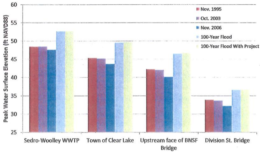
Figure 8: Comparison of Modeled Peak Water Levels in Historic and 100-Year Floods
