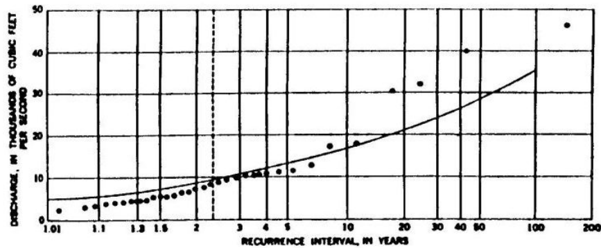
FIGURE 10.—Frequency of annual floods, Cascade River at Marblemount, Wash.
