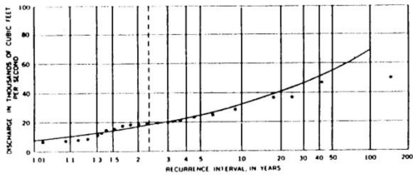
FIGURE 12.—Frequency of annual floods, Baker River below Anderson Creek near Concrete, Wash.
