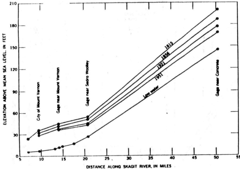
FIGURE 5.—Flood profiles.
