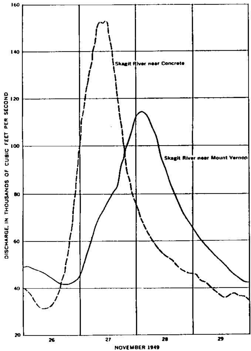
FIGURE 1.—Hydrographs of short-duration flood peaks.
