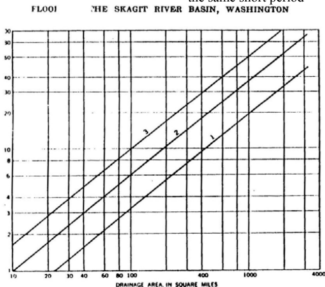
FIGURE 8.—Variation of mean annual flood with drainage area.
