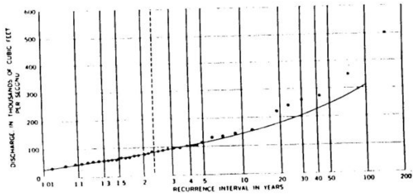
FIGURE 13.—Frequency of annual floods, Skagit River near Concrete, Wash.
