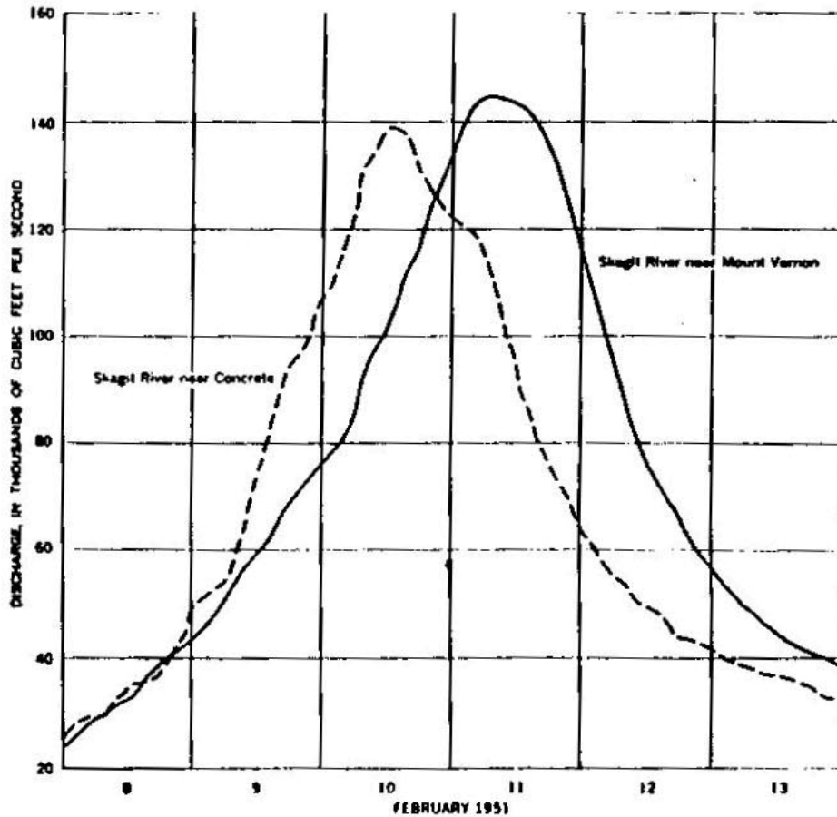
FIGURE 2.—Hydrographs of long-duration flood peaks.
