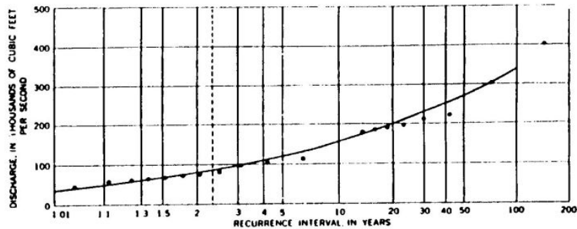
FIGURE 14.—Frequency of annual floods, Skagit River near Sedro Woolley, Wash.
