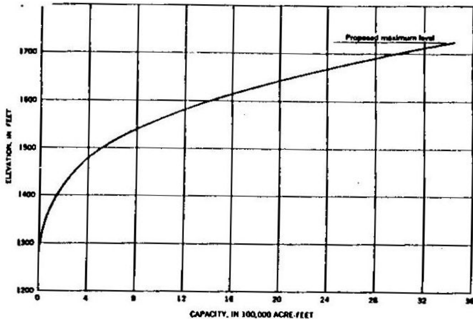
FIGURE 3.—Capacity curve for Ross Reservoir.
