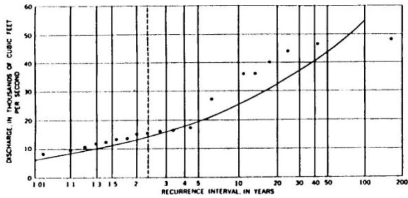
FIGURE 11.—Frequency of annual floods, Sauk River at Darrington, Wash.
