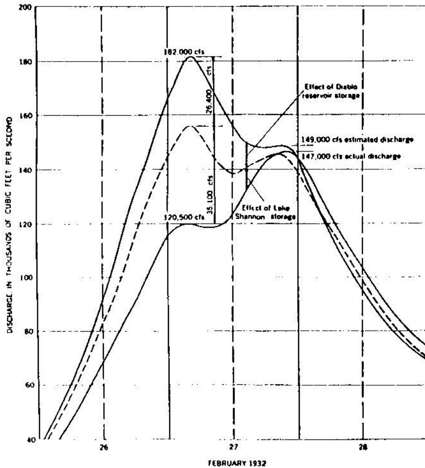
FIGURE 4.—Hydrographs showing effect of dams on flood peak.
