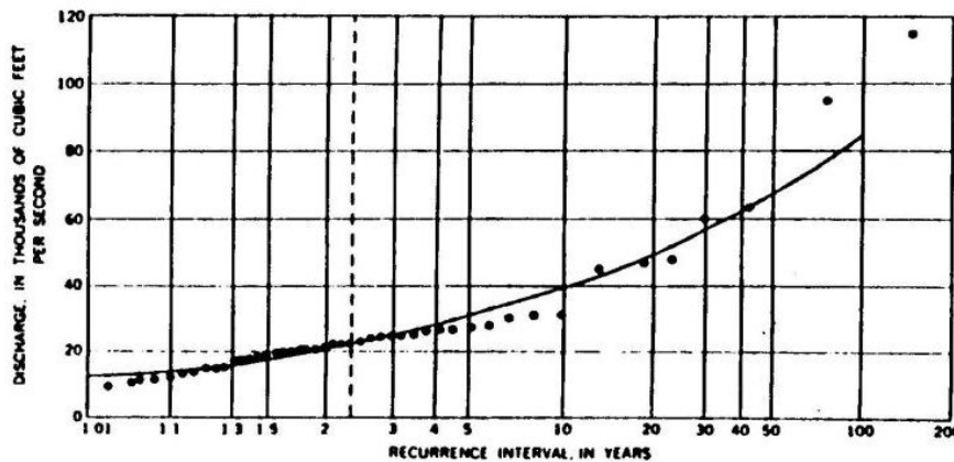
FIGURE 9.—Frequency of annual floods, Skagit River at Newhalom, Wash.
