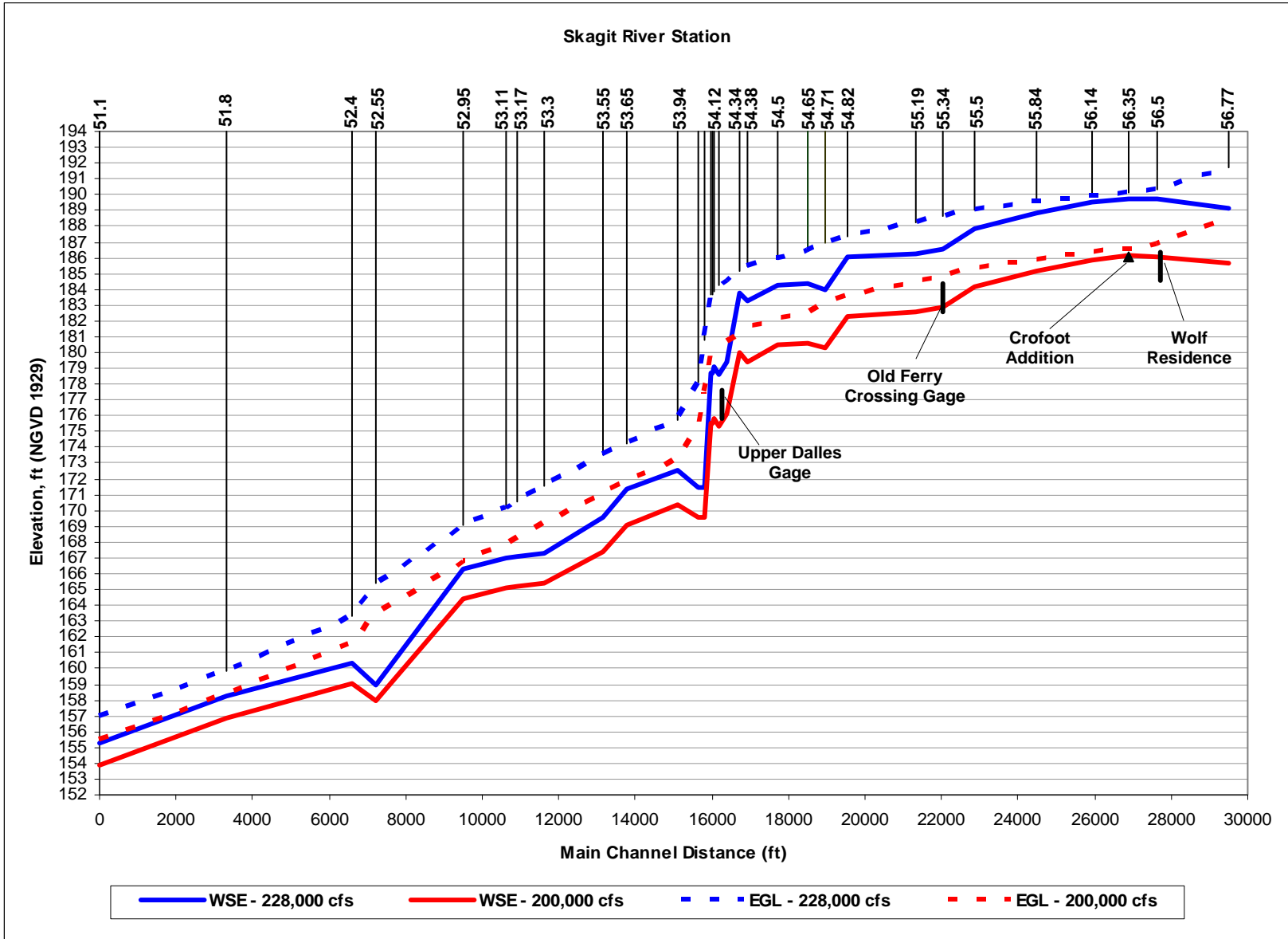
Figure 9. 1921 Model Flood Profiles – Low Expansion/Contraction Coefficients
