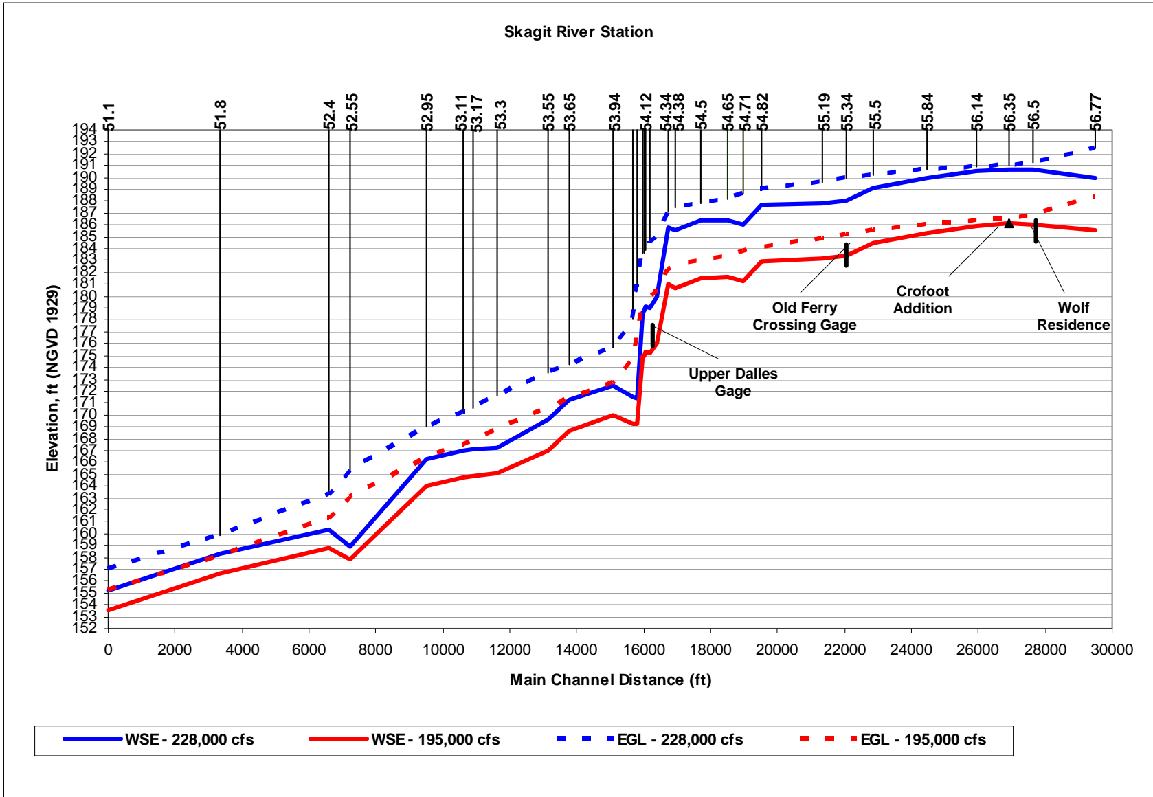
Figure 12. Final 1921 Model Water Surface Profiles.
