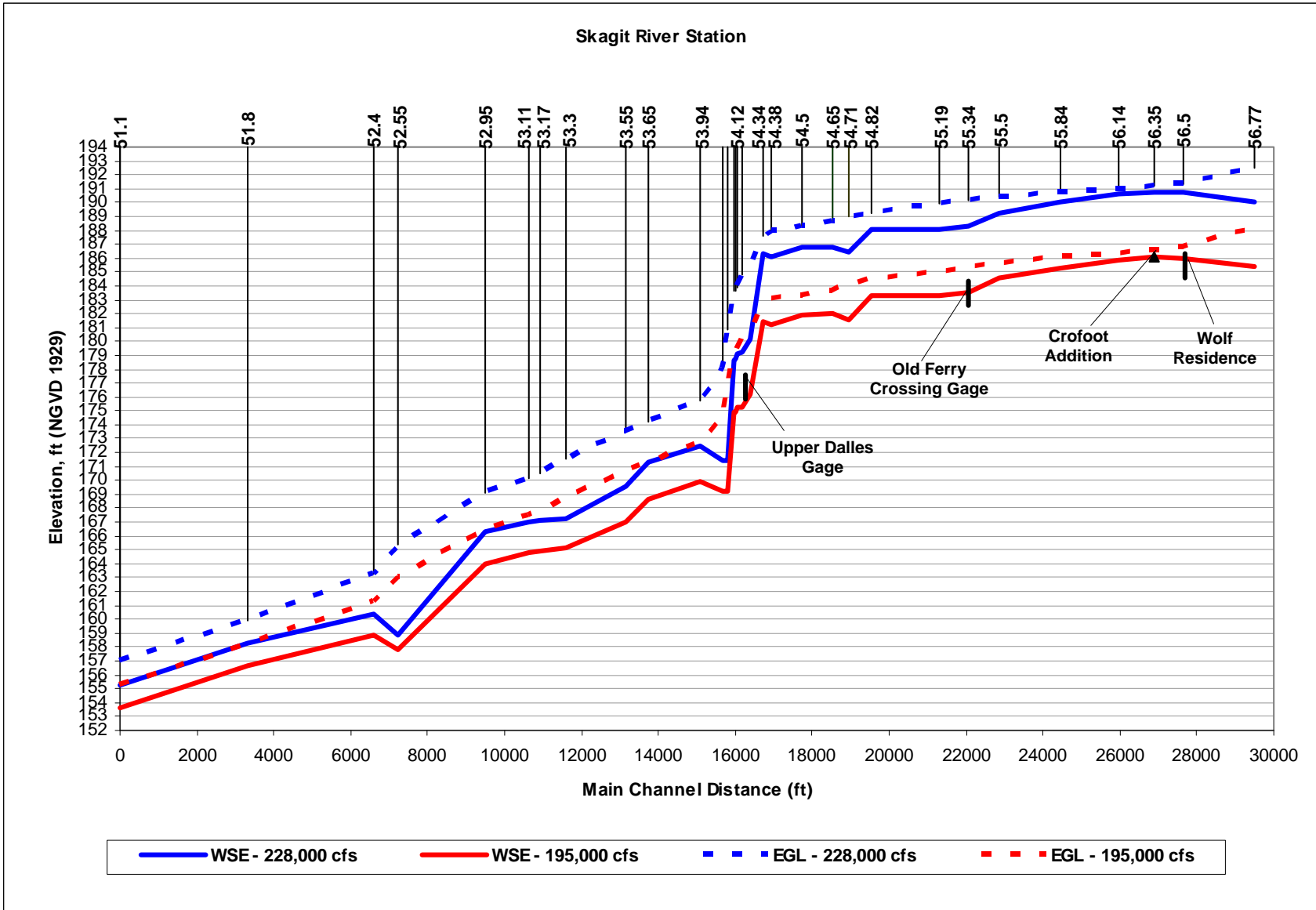
Figure 8. 1921 Model Flood Profiles – High Expansion/Contraction Coefficient
